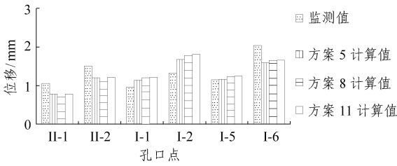
图 6 开挖完成后方案 5, 8, 11 计算位移与监测位移对比 Fig.6 Comparison of the calculated displacements of scheme 5, 8, 11 and monitored displacements after the third step of excavation
