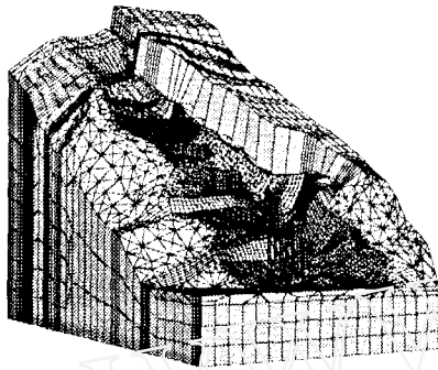
图 3 加固计算模型 (去掉了滑体和滑带单元) Fig.3 Model for reinforcing simulation (elements in sliding body and surface are removed)
