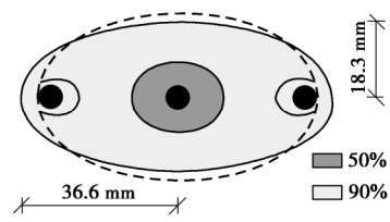
图 5 三针式探头测试介质范围计算结果 Fig. 5 Computed sampling area of three-rod probe
