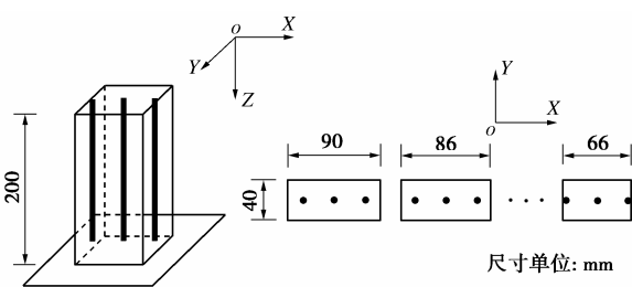
图 7 X 方向测试范围试验装置 Fig. 7 Experimental equipment for measuring sampling area in X direction
