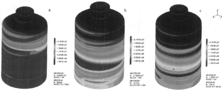
图 9 不同时刻主容器结构的等效应力图 Fig. 9 Stress figure at different time of main vessel 时刻, s: a—1.700; b—1.940; c—2.340
