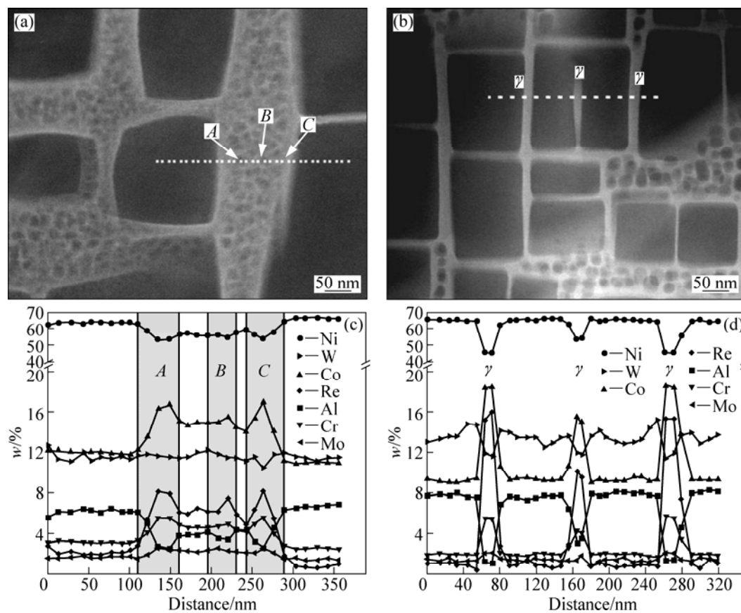
Fig. 3 Dark-field STEM micrographs of \gamma/\gamma' microstructures after the first-step aging (a) and the second-step aging for 25 h (b), composition profiles (c), (d) along white lines in (a) and (b), respectively
