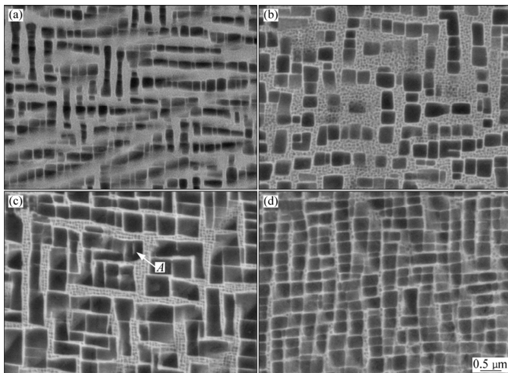
Fig. 2 BSE micrographs of \gamma/\gamma' microstructures after the first-step (a) and the second-step aging for 25 h (b), 35 h (c) and 40 h (d) (Bright area is \gamma matrix and dark area is \gamma' phase)
