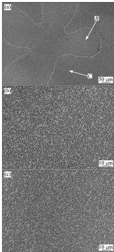
Fig. 1 BSE micrographs of as-grown crystals: (a) Low-magnification image showing weak dendrite pattern (boundary of dendrite is sketched by dotted lines); (b) \gamma/\gamma' microstructure in dendrite cores; (c) \gamma/\gamma' microstructure in interdendritic regions
